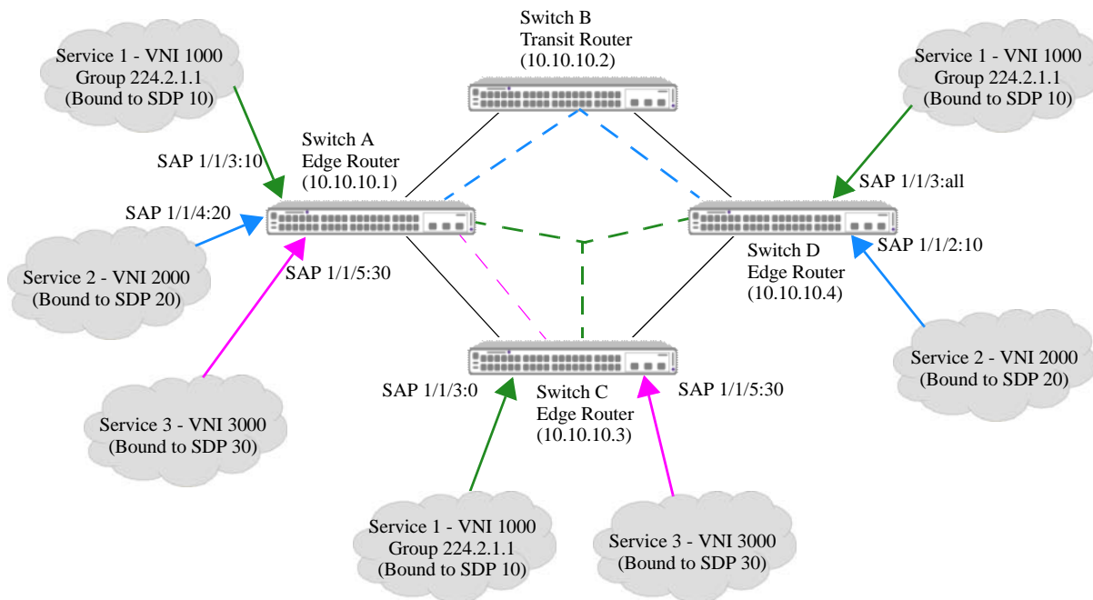
Figure 3: Example 1 VXLAN Configuration
